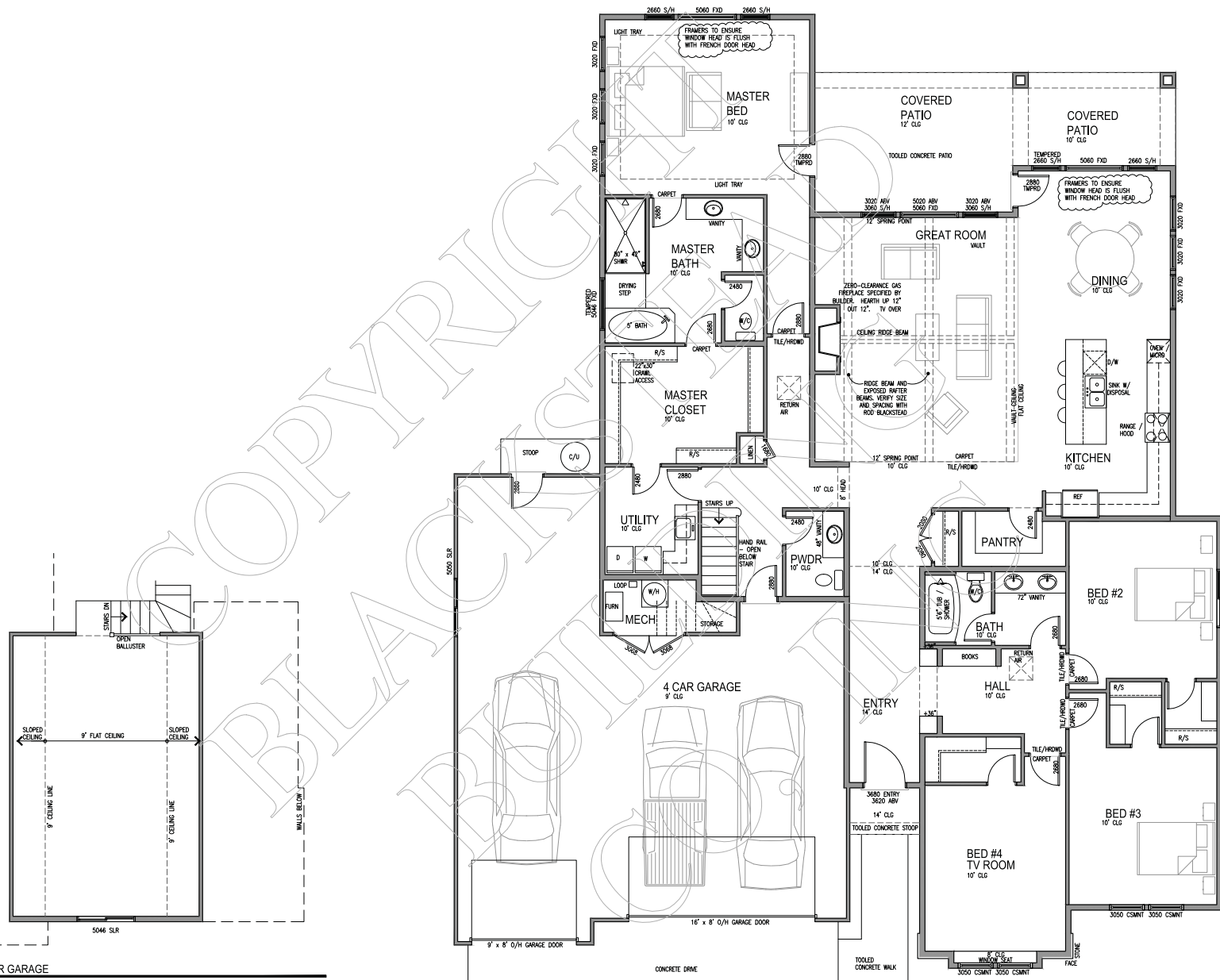
1 FLOOR PLAN - NOTED 1/4" = 1'-0"
